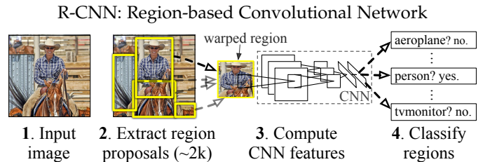
Fig. 1. Object detection system overview. Our system (1) takes an input image, (2) extracts around 2000 bottom-up region proposals, (3) computes features for each proposal using a large convolutional network (CNN), and then (4) classifies each region using class-specific linear SVMs. We trained an R-CNN that achieves a mean average precision (mAP) of 62.9% on PASCAL VOC 2010. For comparison, [21] reports 35.1% mAP using the same region proposals, but with a spatial pyramid and bag-of-visual-words approach. The popular deformable part models perform at 33.4%. On the 200-class ILSVRC2013 detection dataset, we trained an R-CNN with a mAP of 31.4%, a large improvement over OverFeat [19], which had the previous best result at 24.3% mAP.
