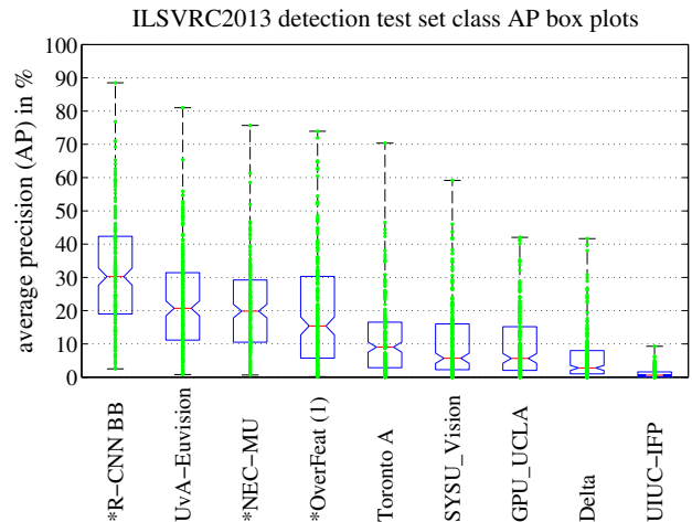
Fig. 3. (Left) Mean average precision on the ILSVRC2013 detection test set. Methods preceded by * use outside training data (images and labels from the ILSVRC classification dataset in all cases). (Right) Box plots for the 200 average precision values per method. A box plot for the post-competition OverFeat result is not shown because per-class APs are not yet available. The red line marks the median AP, the box bottom and top are the 25th and 75th percentiles. The whiskers extend to the min and max AP of each method. Each AP is plotted as a green dot over the whiskers (best viewed digitally with zoom).
