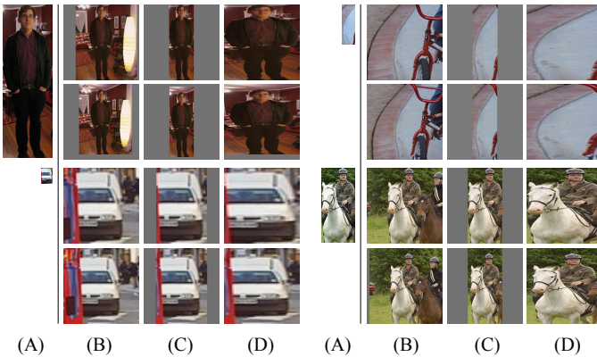
Fig. 7. Different object proposal transformations. (A) the original object proposal at its actual scale relative to the transformed CNN inputs; (B) tightest square with context; (C) tightest square without context; (D) warp. Within each column and example proposal, the top row corresponds to p = 0 pixels of context padding while the bottom row has p = 16 pixels of context padding.
