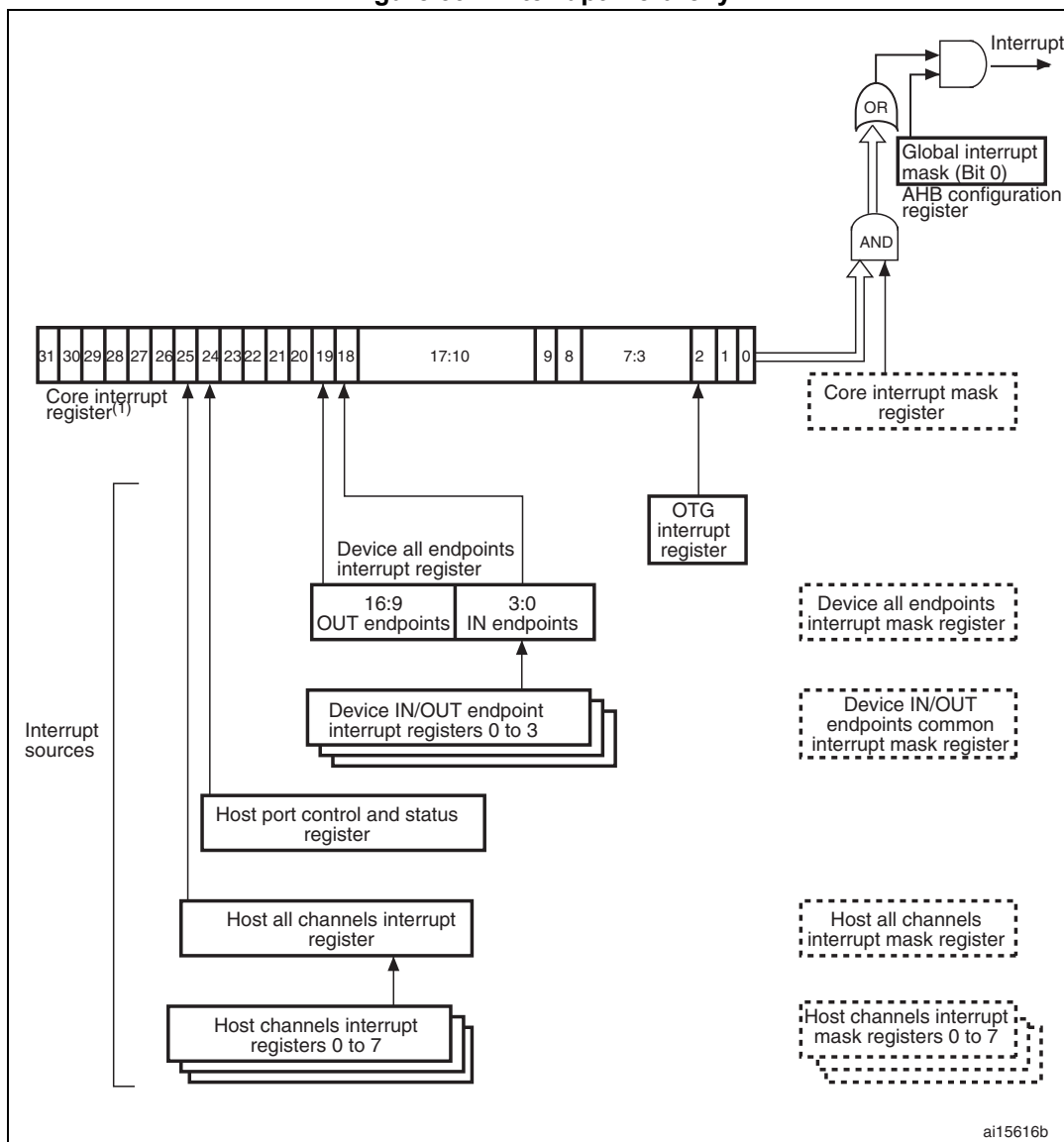
Figure 394. Interrupt hierarchy
