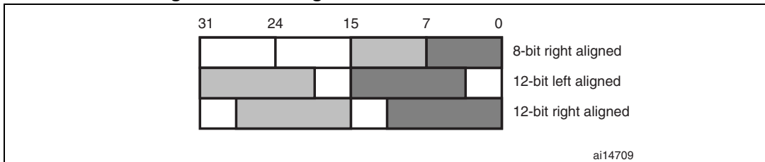
Figure 66. Data registers in dual DAC channel mode
