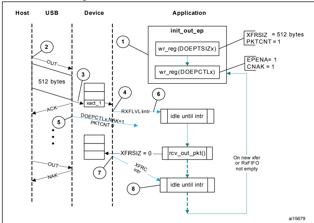
Figure 426. Slave mode bulk OUT transaction
