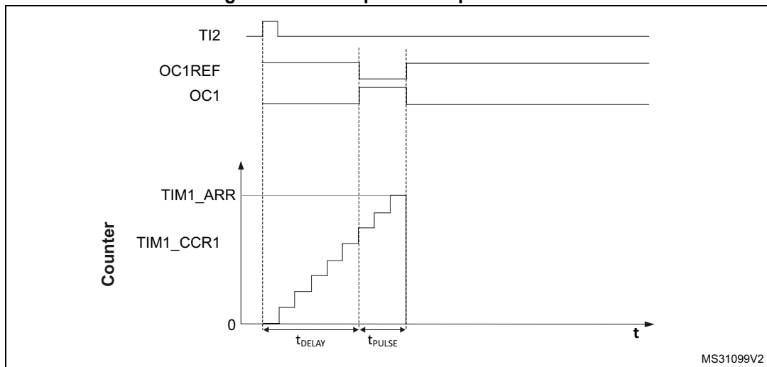
Figure 126. Example of one pulse mode.
