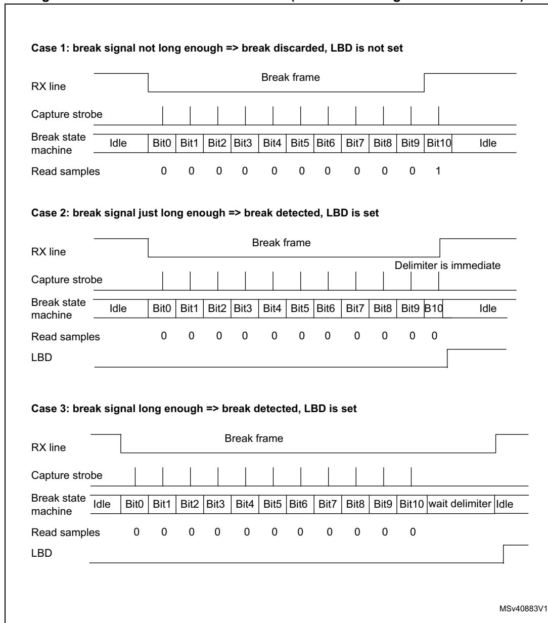
Figure 305. Break detection in LIN mode (11-bit break length - LBDL bit is set)
