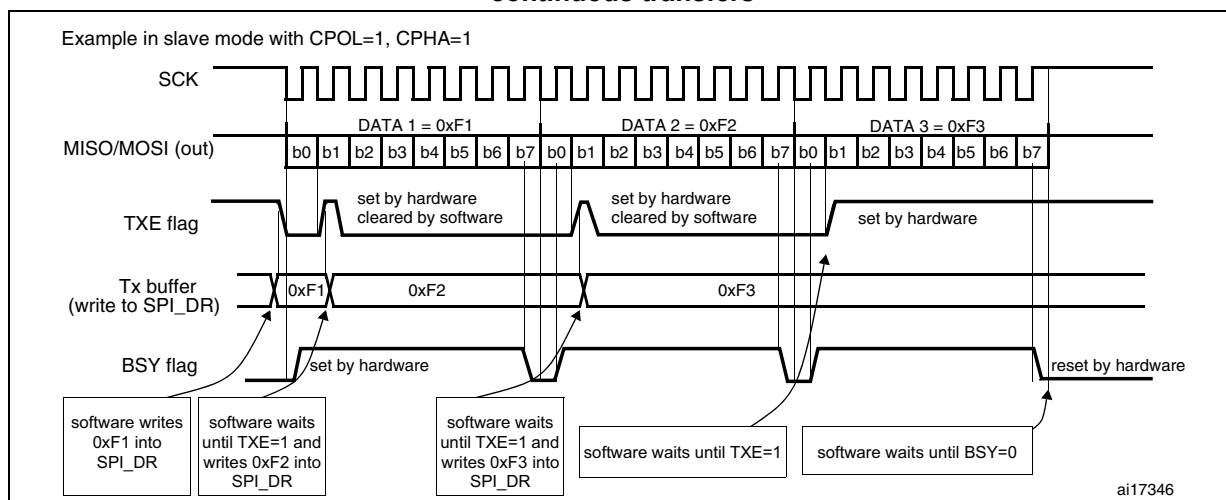
Figure 256. TXE/BSY in Slave transmit-only mode (BIDIMODE=0 and RXONLY=0) in case of continuous transfers
