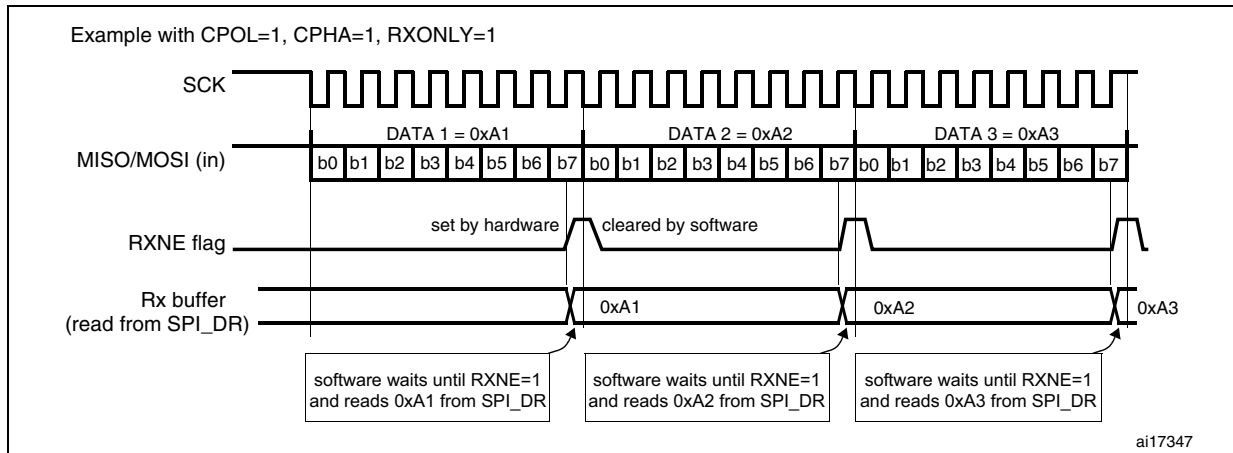
Figure 257. RXNE behavior in receive-only mode (BIDIRMODE=0 and RXONLY=1) in case of continuous transfers
