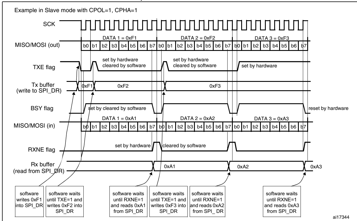
Figure 254. TXE/RXNE/BSY behavior in Slave / full-duplex mode (BIDIMODE=0, RXONLY=0) in case of continuous transfers
