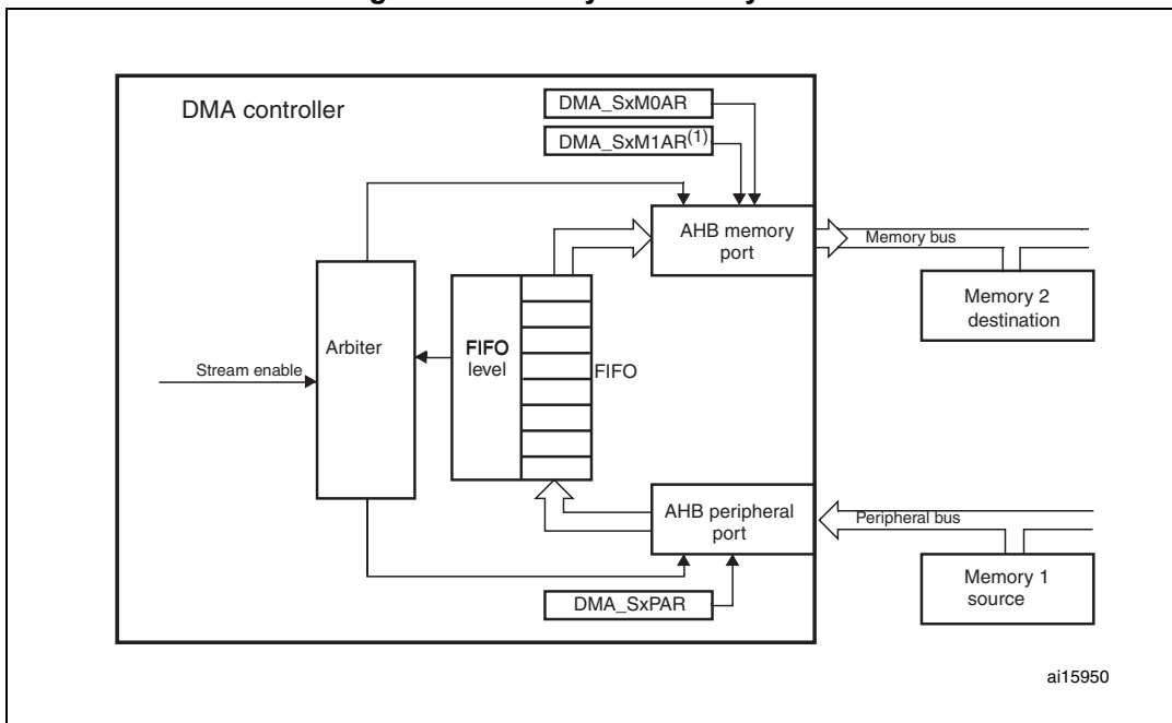
Figure 38. Memory-to-memory mode
