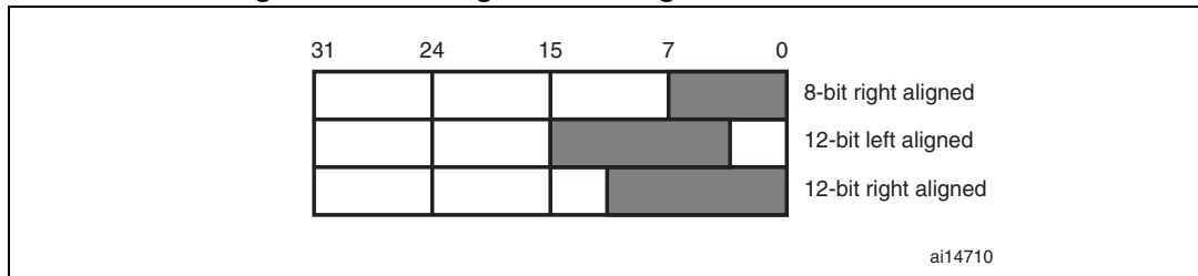
Figure 65. Data registers in single DAC channel mode
