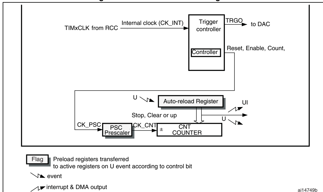
Figure 203. Basic timer block diagram
