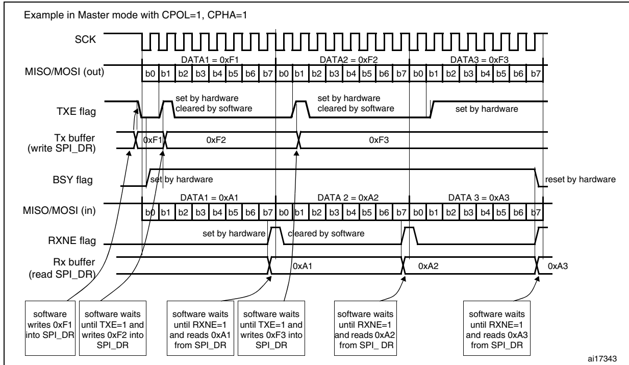
Figure 253. TXE/RXNE/BSY behavior in Master / full-duplex mode (BIDIMODE=0 and RXONLY=0) in case of continuous transfers
