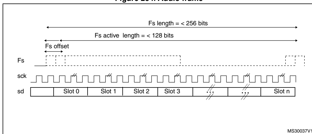
Figure 284. Audio frame
