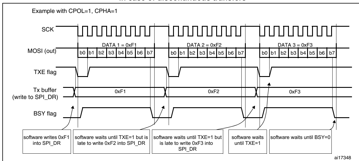
Figure 258. TXE/BSY behavior when transmitting (BIDIRMODE=0 and RXONLY=0) in case of discontinuous transfers
